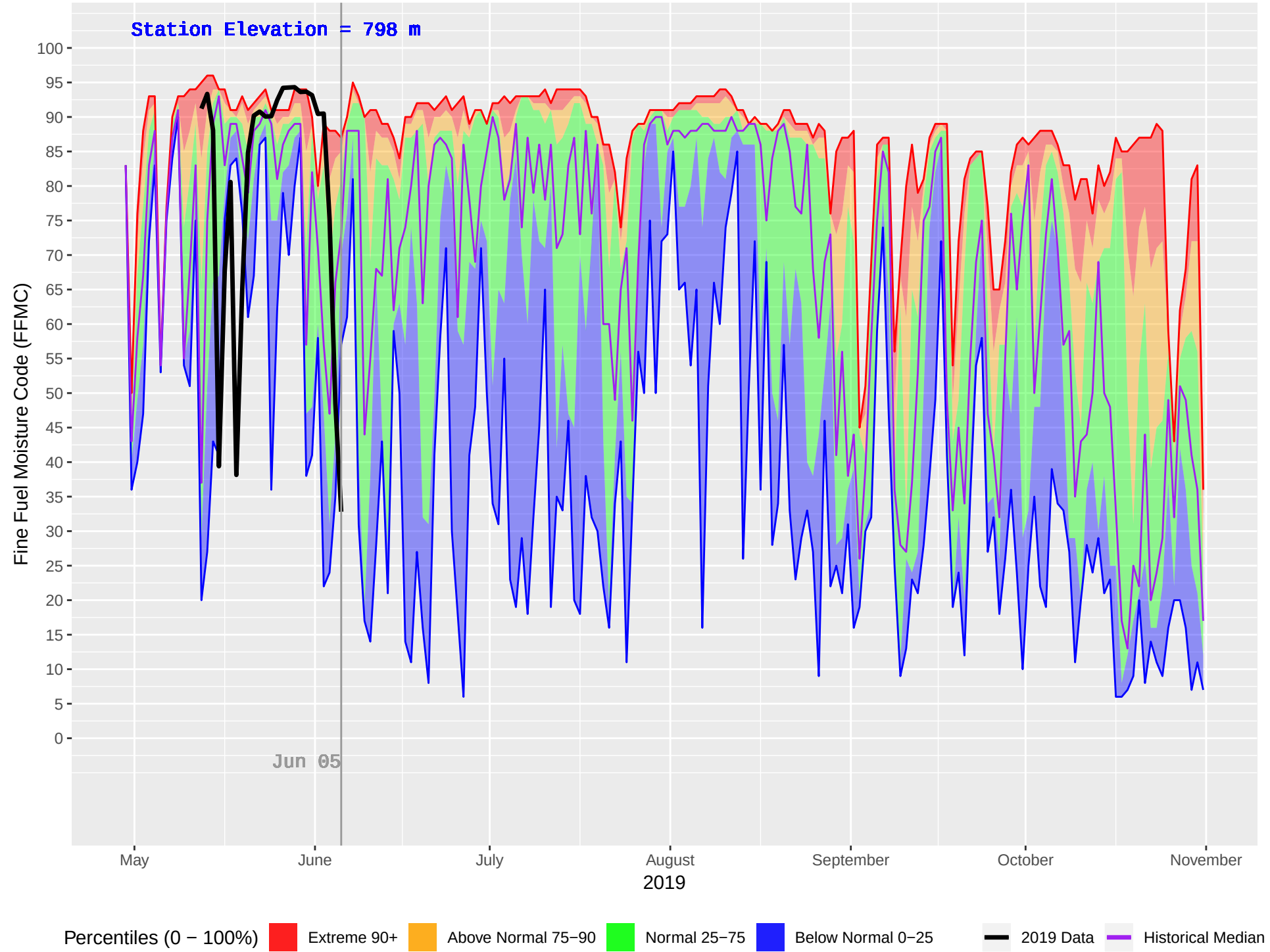
SEVEREID (1165) : Historical (2014–2018) and Current (2019) Daily Fine Fuel Moisture Code (FFMC)
