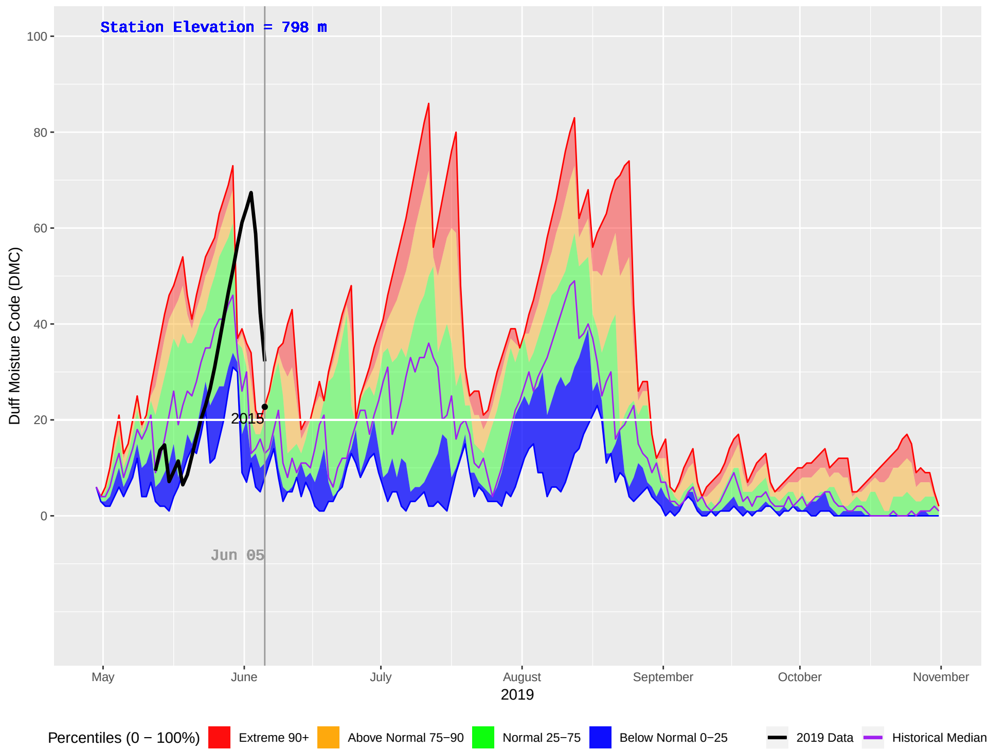
SEVEREID (1165) : Historical (2014–2018), Current (2019) Daily Duff Moisture Code (DMC)
