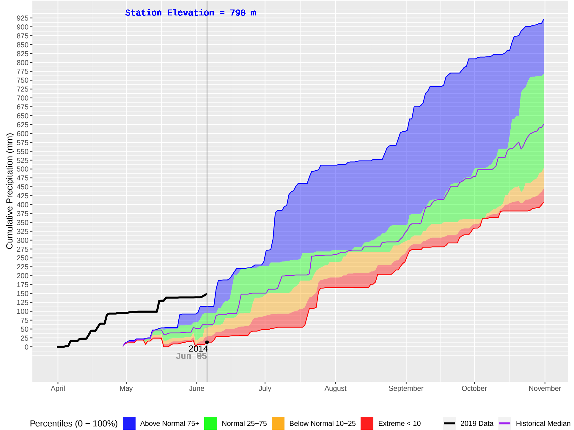
SEVEREID (1165) : Historical (2014–2018), Current (2019) Daily Cumulative Precipitation
