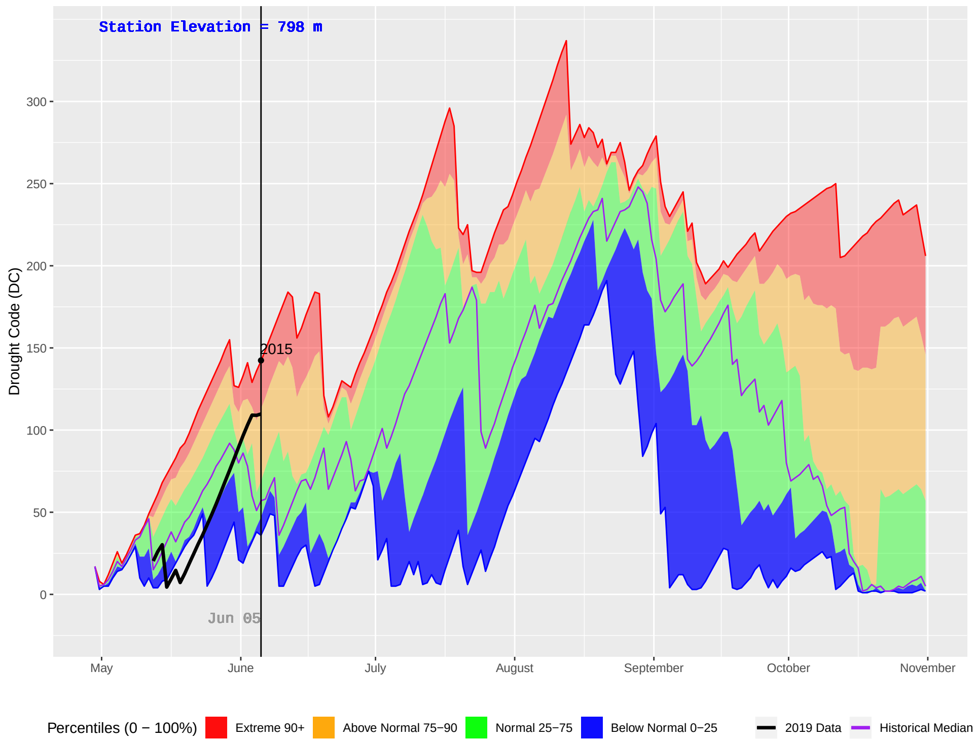
SEVEREID (1165) : Historical (2014–2018) and Current (2019) Daily Drought Code (DC)
